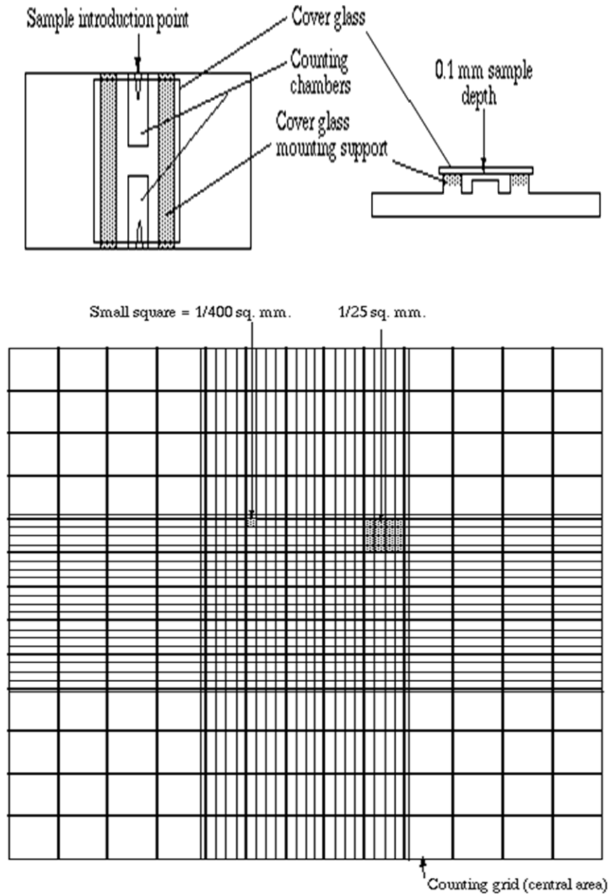
Gambar 4.1 Counting Chamber
