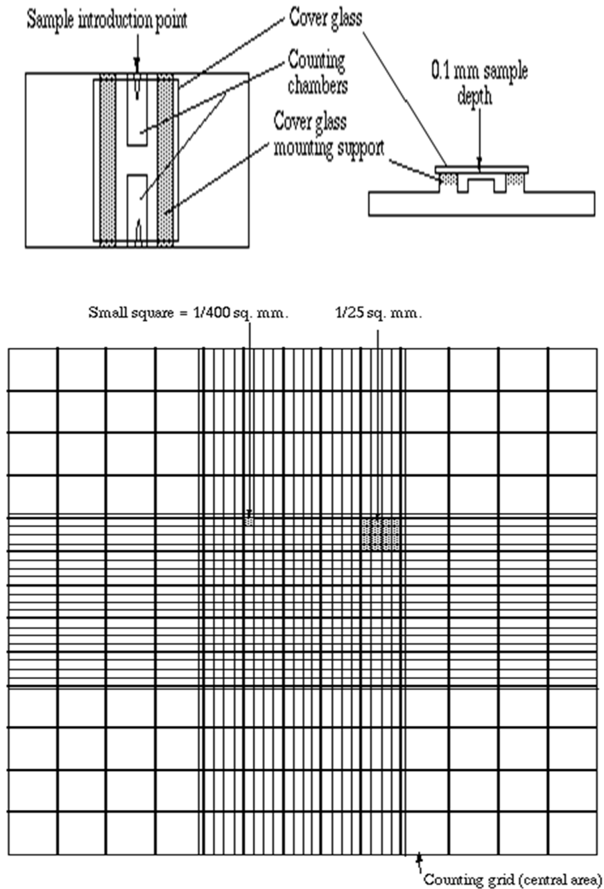
Gambar 4.1 Counting Chamber
