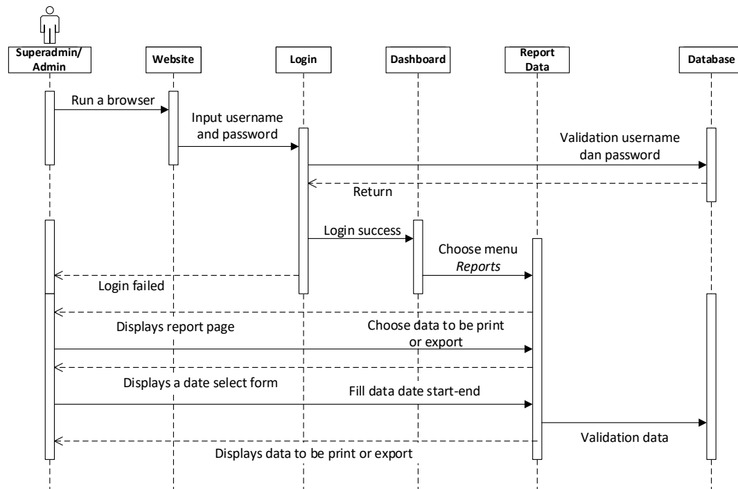
Fig. 9. Sequence Diagram of Data Report
