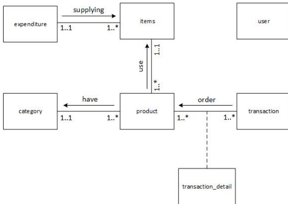
Fig. 10. The Entity-Relationship Diagram of POS System in InHome Café
