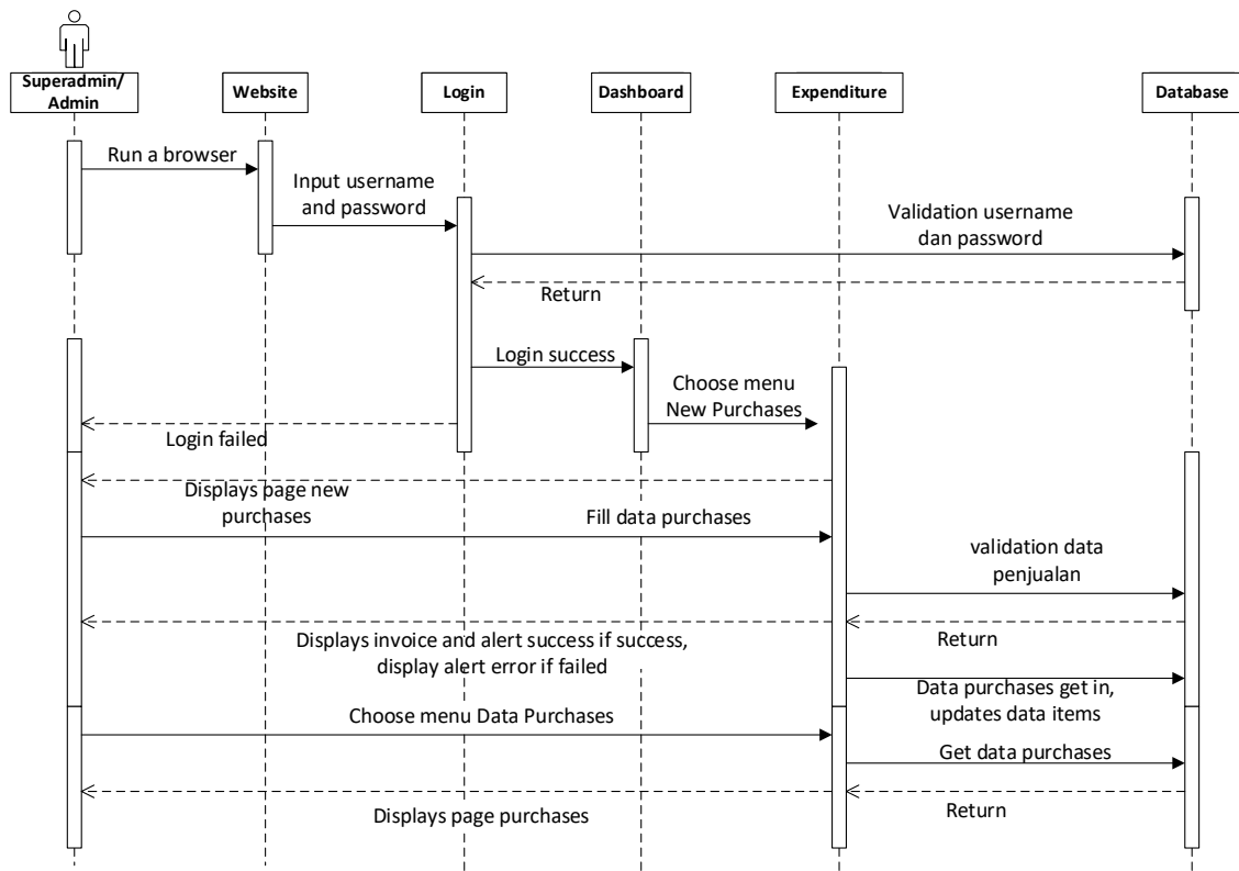
Fig. 8. Sequence Diagram of Purchase
