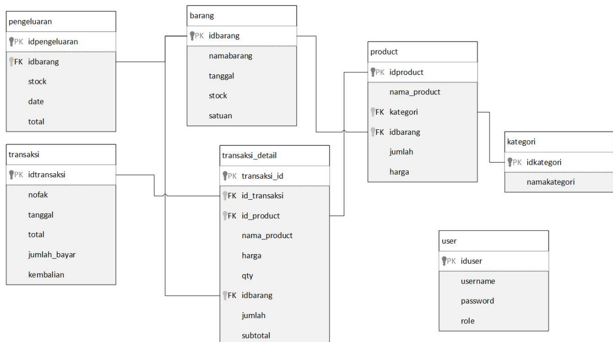
Fig. 11. The Table Relationship Diagram of POS System in InHome Café
