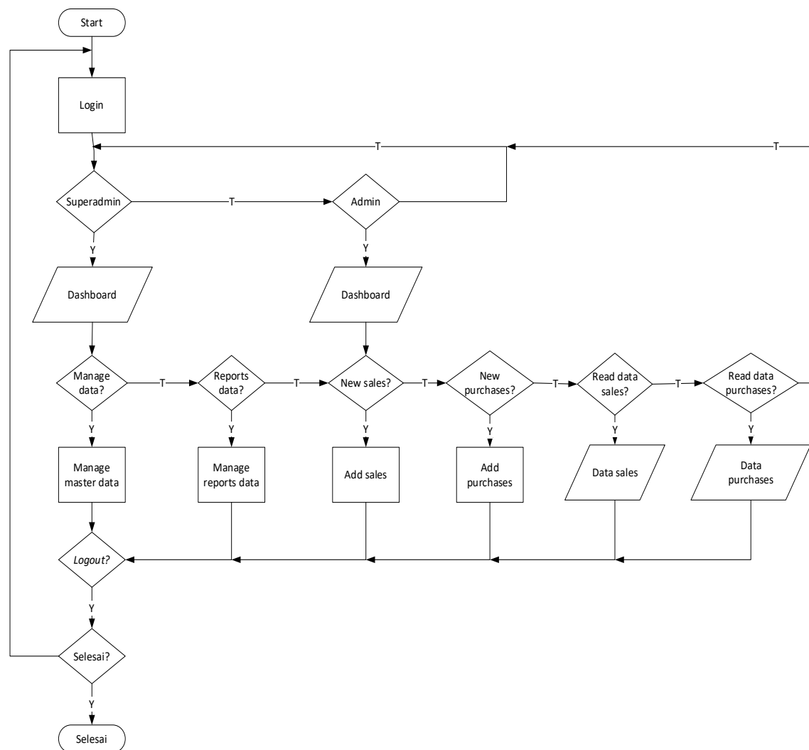
Fig. 5. Flowchart of the Whole POS System in InHome Cafe
