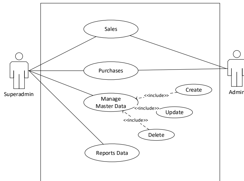
Fig. 6. Usecase POS System in InHome Café
