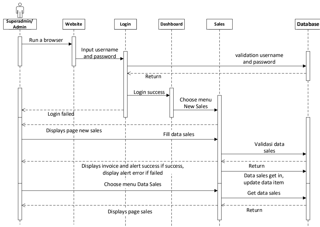
Fig. 7. Sequence Diagram of Sales
