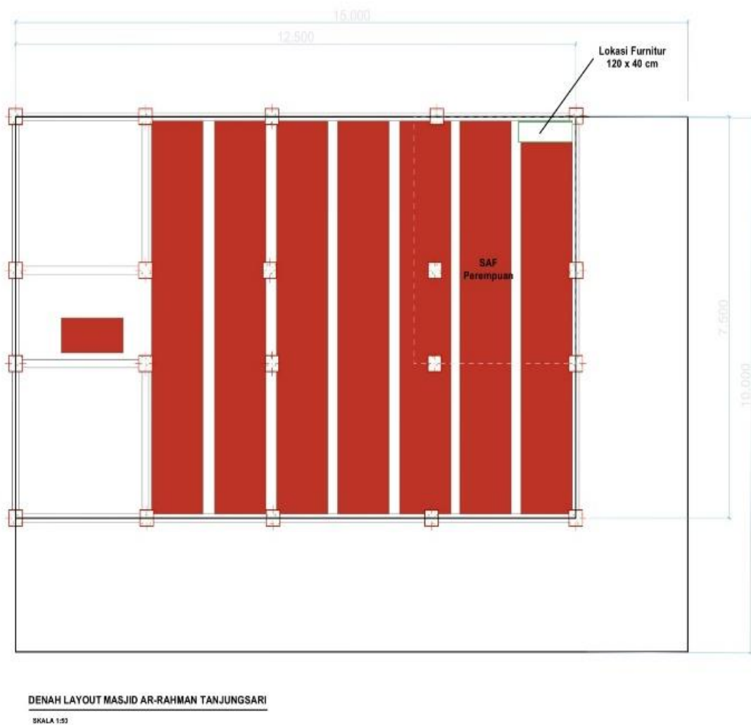
Gambar 3. Layout Masjid Ar-Rahman
