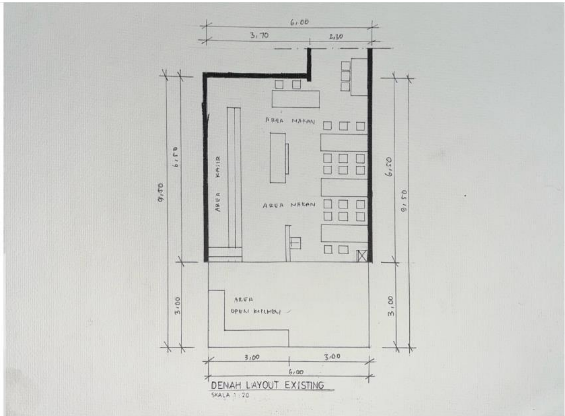
DENAH LAYOUT EXISTING
