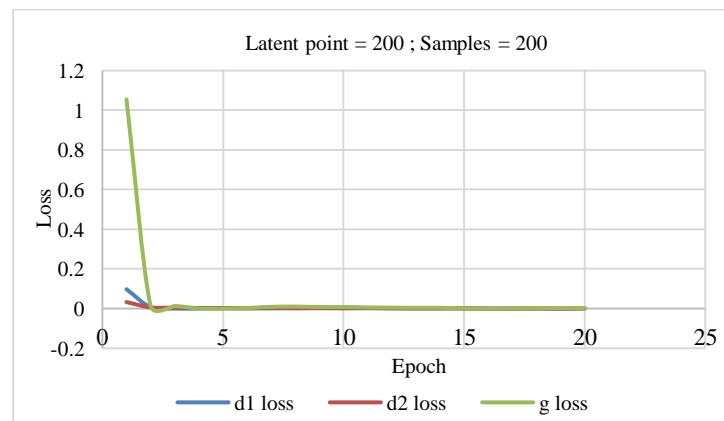
Figure 4. Latent Point = 200 and Samples = 200 (chart)
