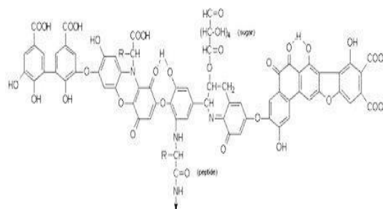
Fig. 1. Structure humic acid (Stevenson,1982)
