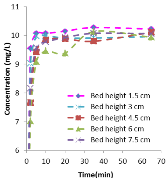
Fig. 4. Continuous adsorption of NOM on humic acid at ozonated time 5 min
