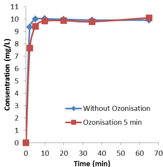
Fig. 5. Breakthrough curve comparison between with and without ozonisation
