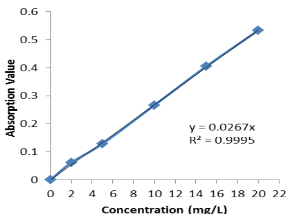
Fig. 2. Standardization curve of humic acid
