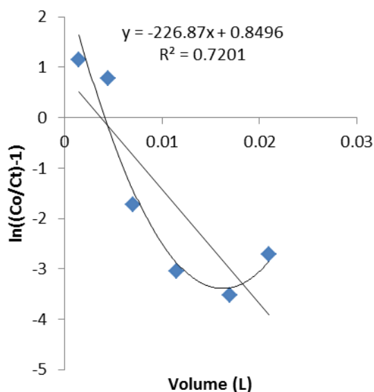
Fig. 6. Linearization curve of Thomas equation at bed height 4.5 cm and ozonated time 5 min
