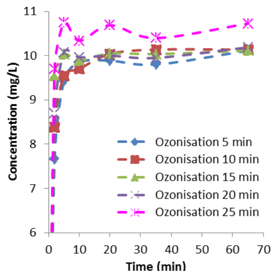
Fig. 3. Continuous adsorption of NOM on humic acid at bed height of 4.5 cm
