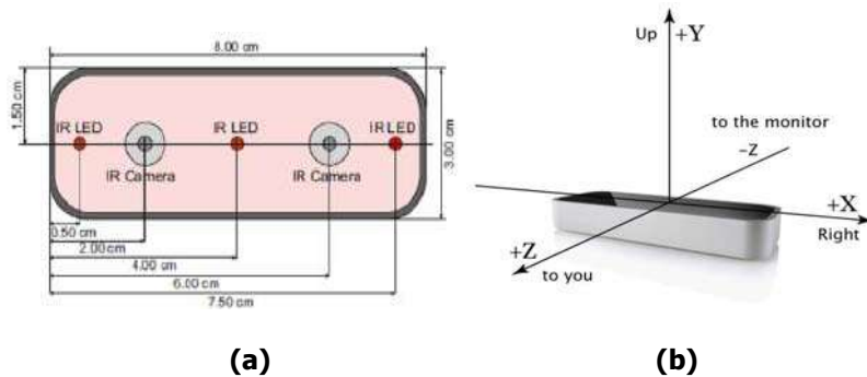
Figure 3. (a) Leap Motion Controller Schematic, (b) Leap Motion Controller (Weichert, 2013)
