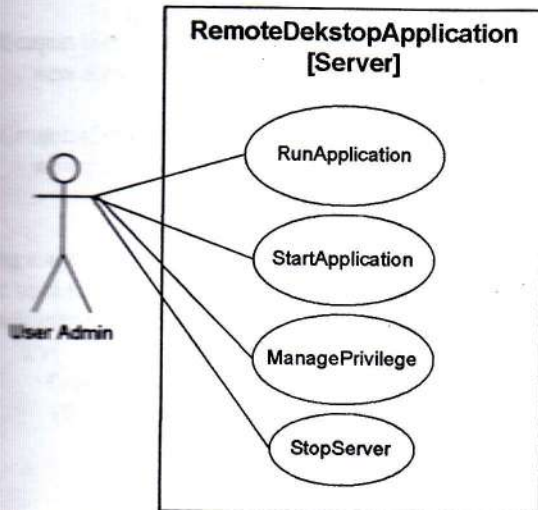
Gambar 2. Use Case Diagram Remote Desktop Server
