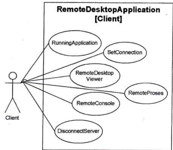
Gambar 3. Use Case Diagram Remote Desktop Client
