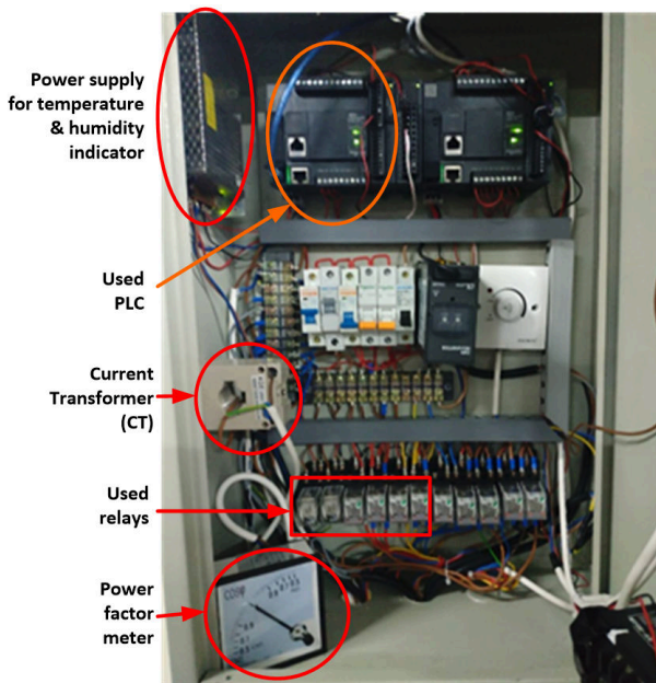
Fig. 4: Realization of the control wiring in a panel box.
