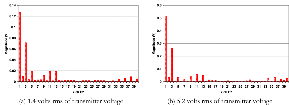
Fig. 29. Frequency spectra of receiver voltage waveforms.
