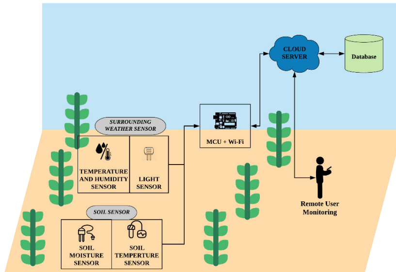
Fig. 1 - Conceptual design
